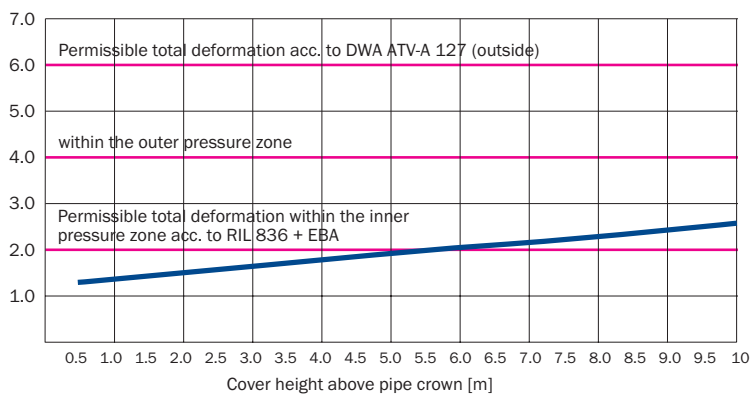
Pipe deformation (SIMODRAIN® PE 100, d=200mm) due to soil load and live load LM 71, multi-track in the case of installation with trench conditions in soil class G1, DPr = 95%
